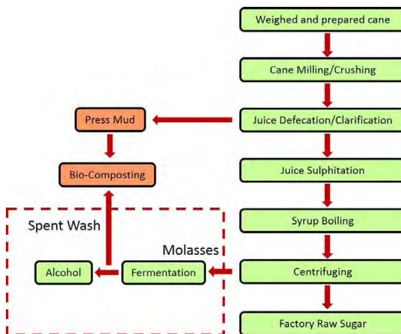
Figure 3-1: Flow chart of press mud generation
